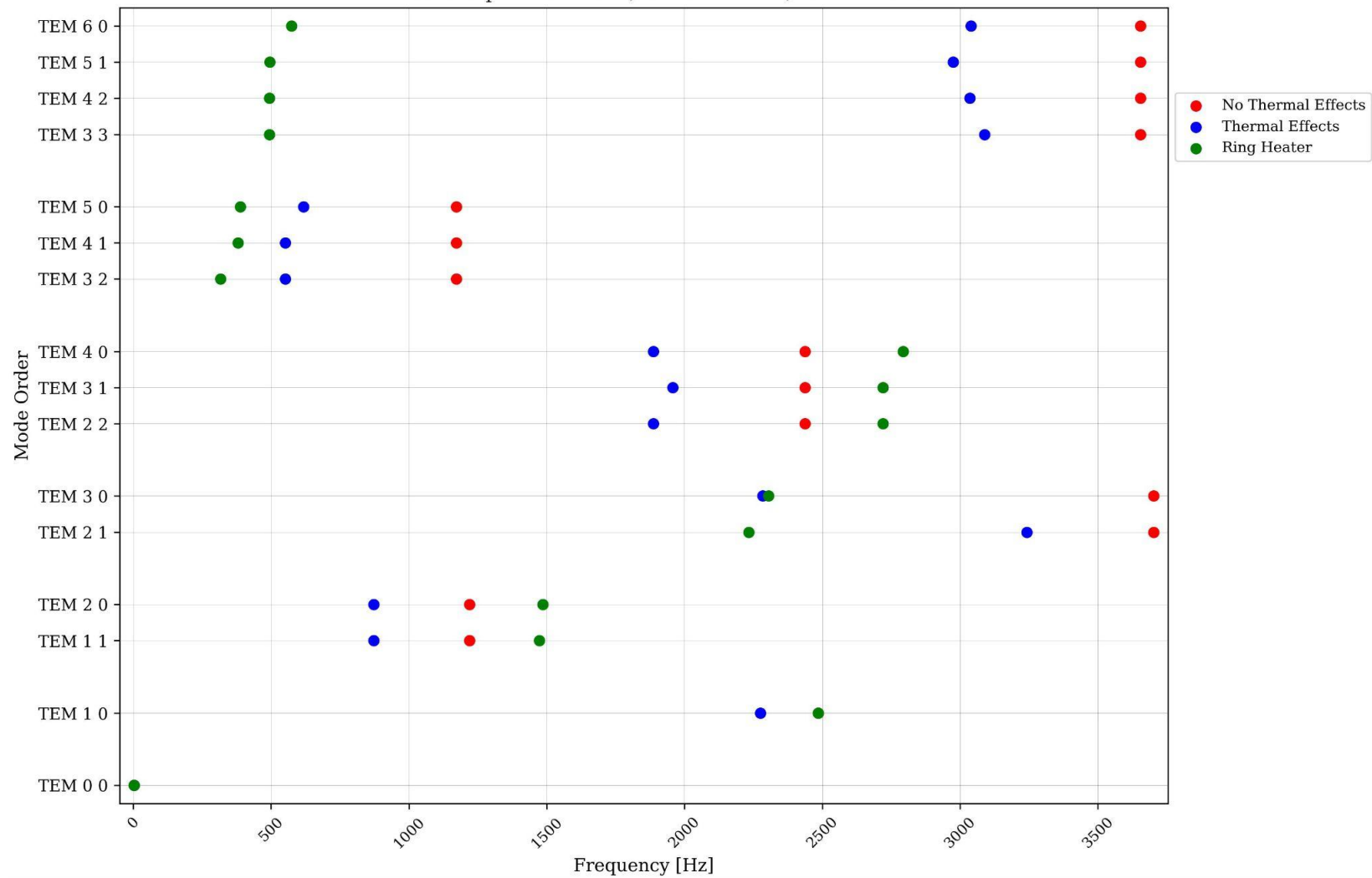
TEM Mode Frequencies 0 to 6, ROC: 26874 m, Beam Size: 0.12
