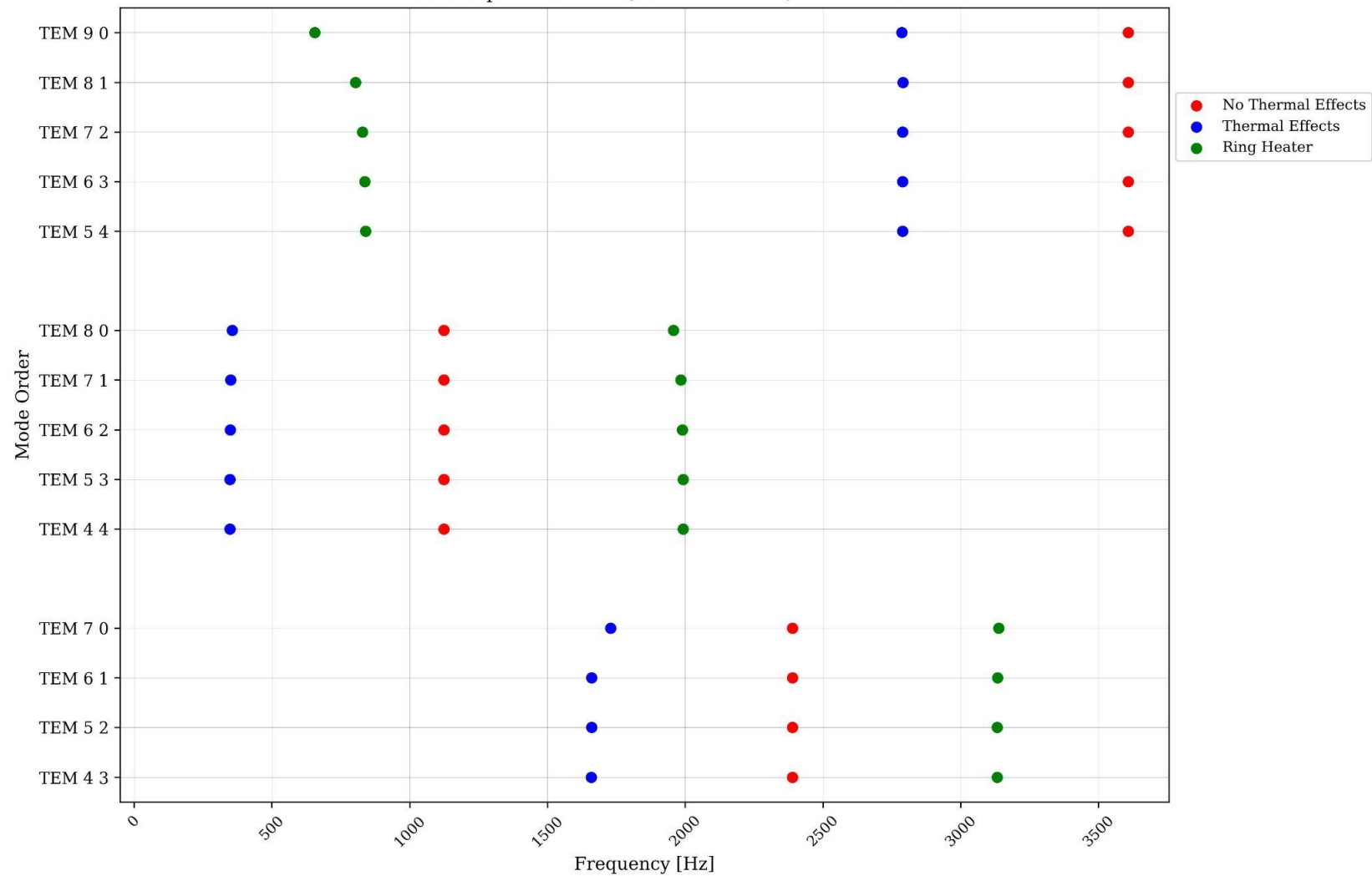
TEM Mode Frequencies 7 to 9, ROC: 26874 m, Beam Size: 0.12
