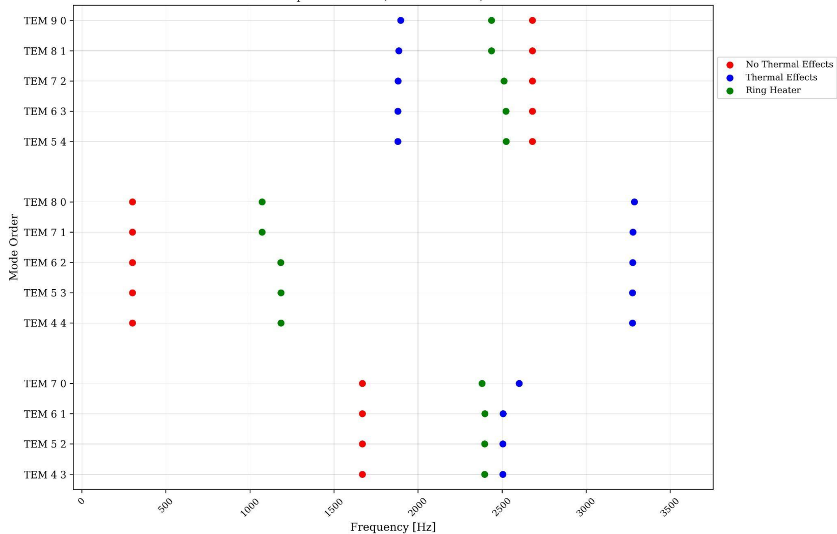
TEM Mode Frequencies 7 to 9, ROC: 28340 m, Beam Size: 0.12
