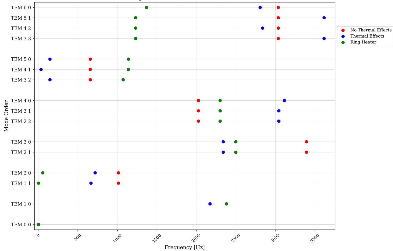
TEM Mode Frequencies 0 to 6, ROC: 28340 m, Beam Size: 0.12
