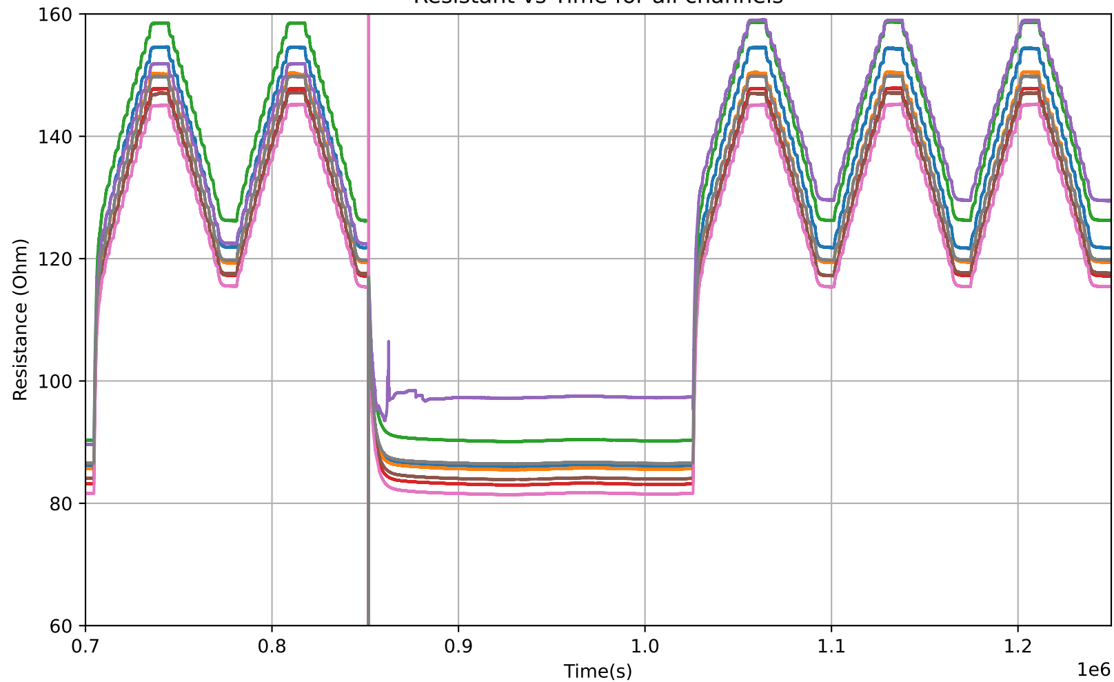
Resistant vs Time for all channels
