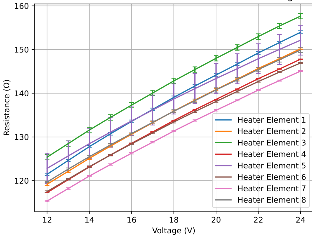
Resistance of Heater Elements as Function of Voltage
