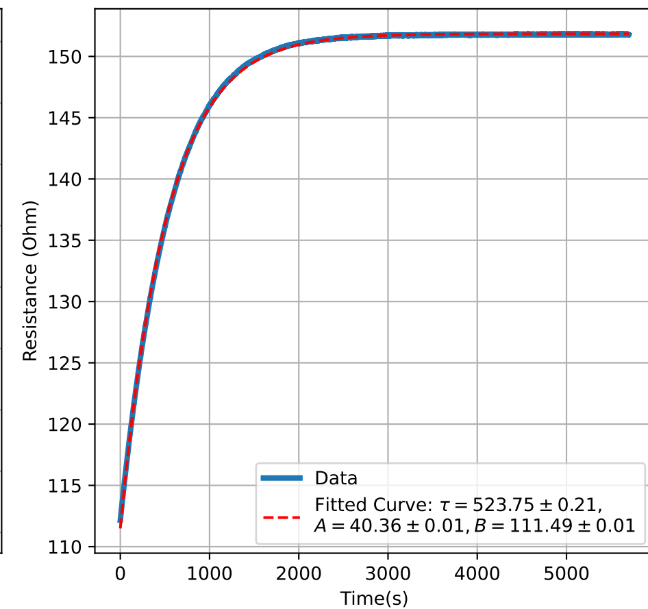
Heater Element 8
