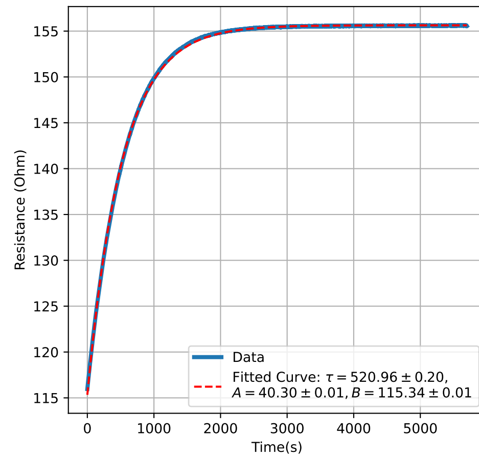
Heater Element 7
