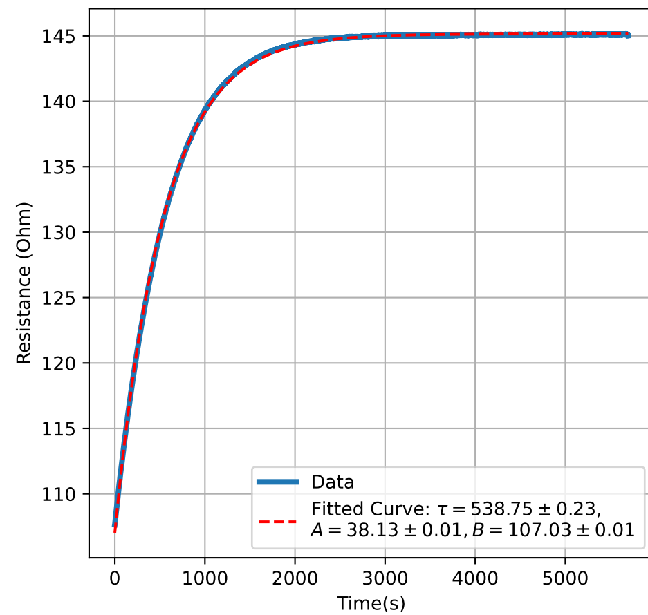
Heater Element 6
