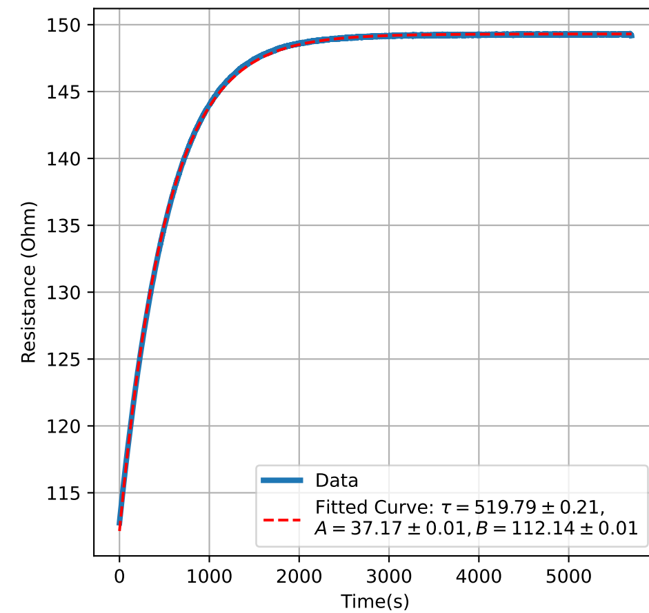
Heater Element 5
