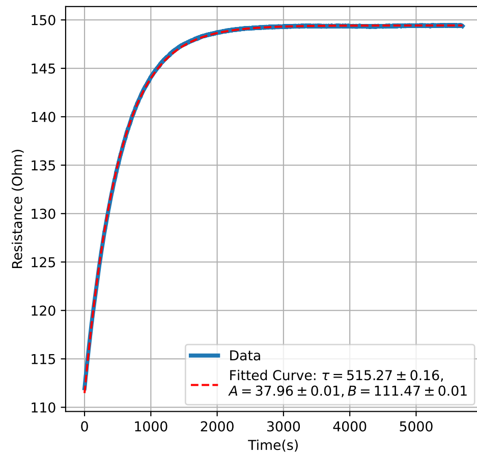
Heater Element 6
