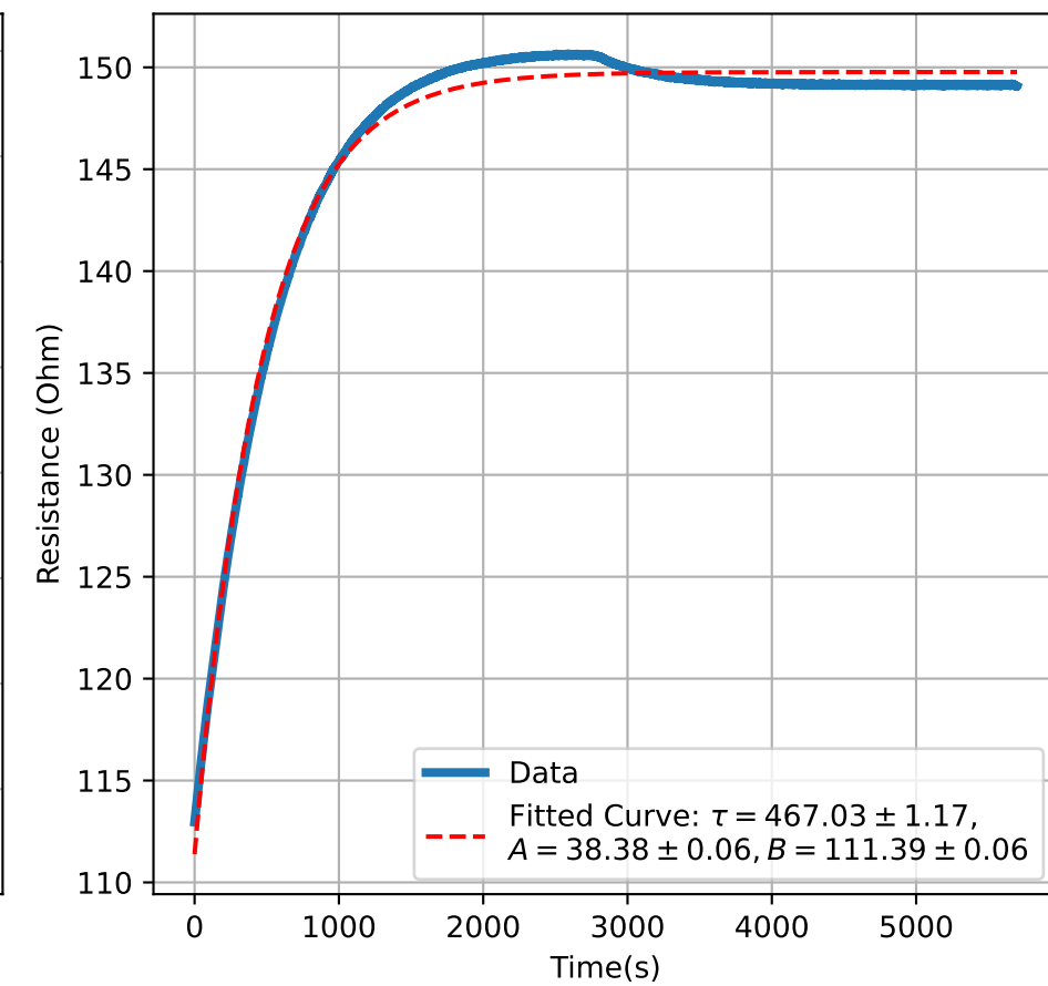
Heater Element 8
