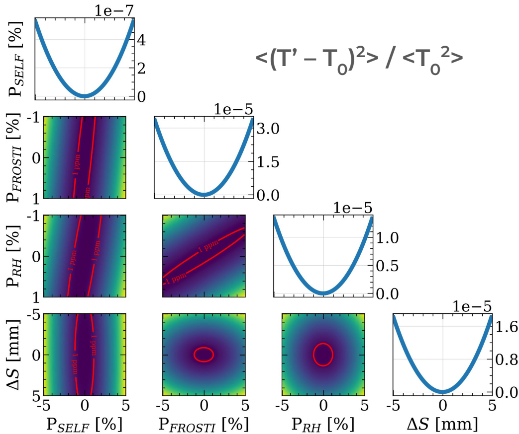
Corner plot showing the correlation between different parameters
