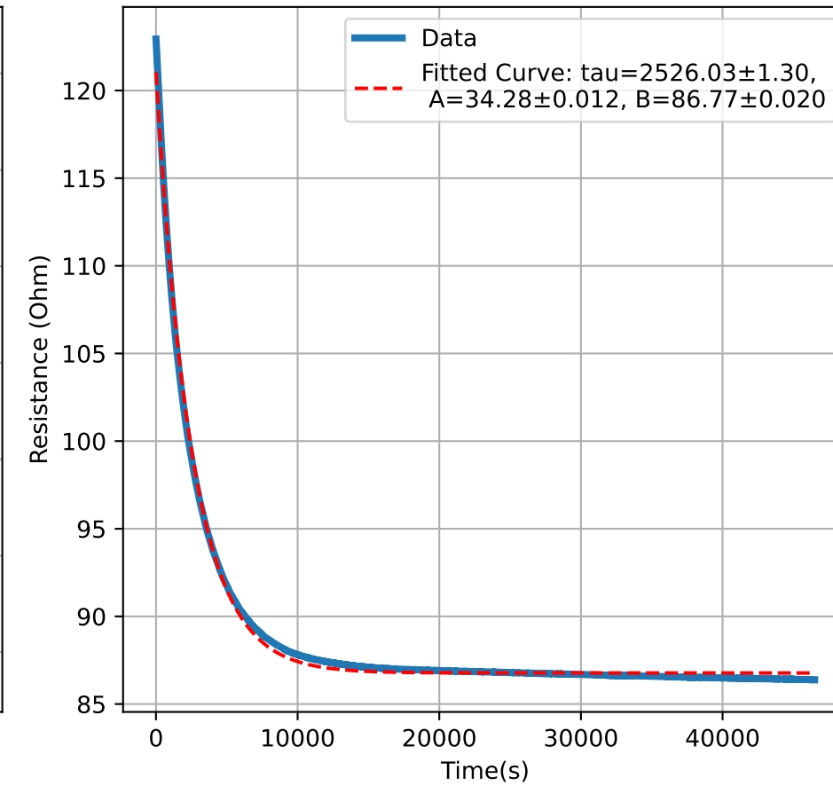
Heater Element 7
