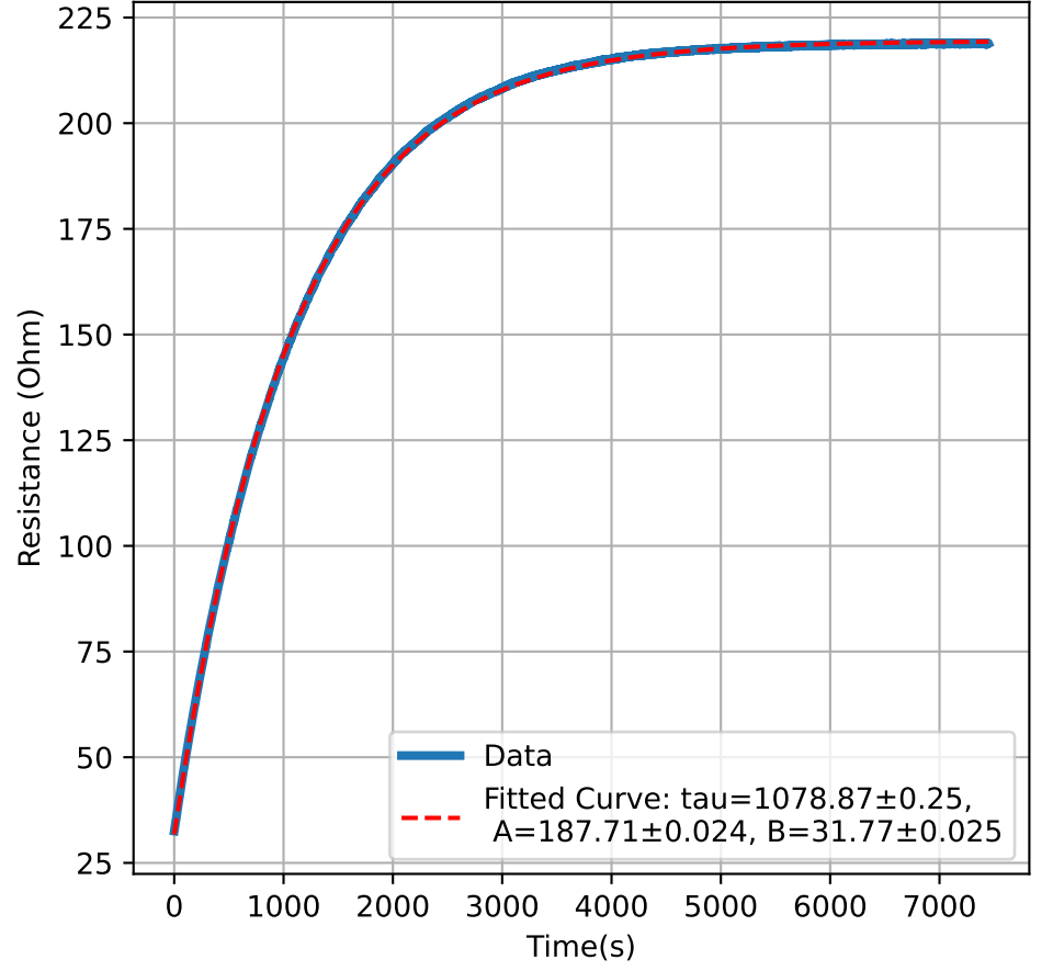
Heater Element 7
