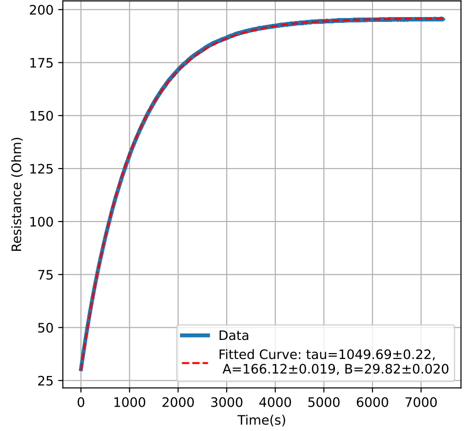
Heater Element 6
