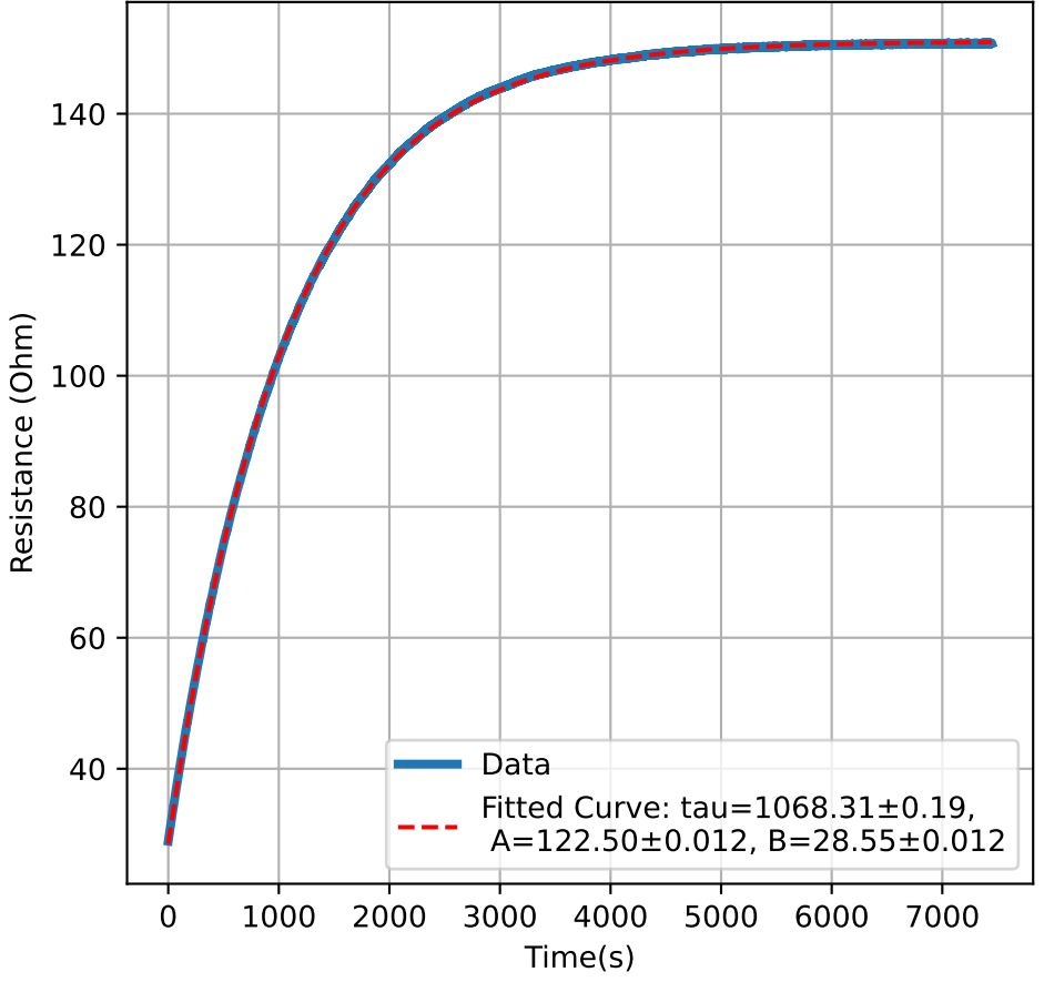
Heater Element 8
