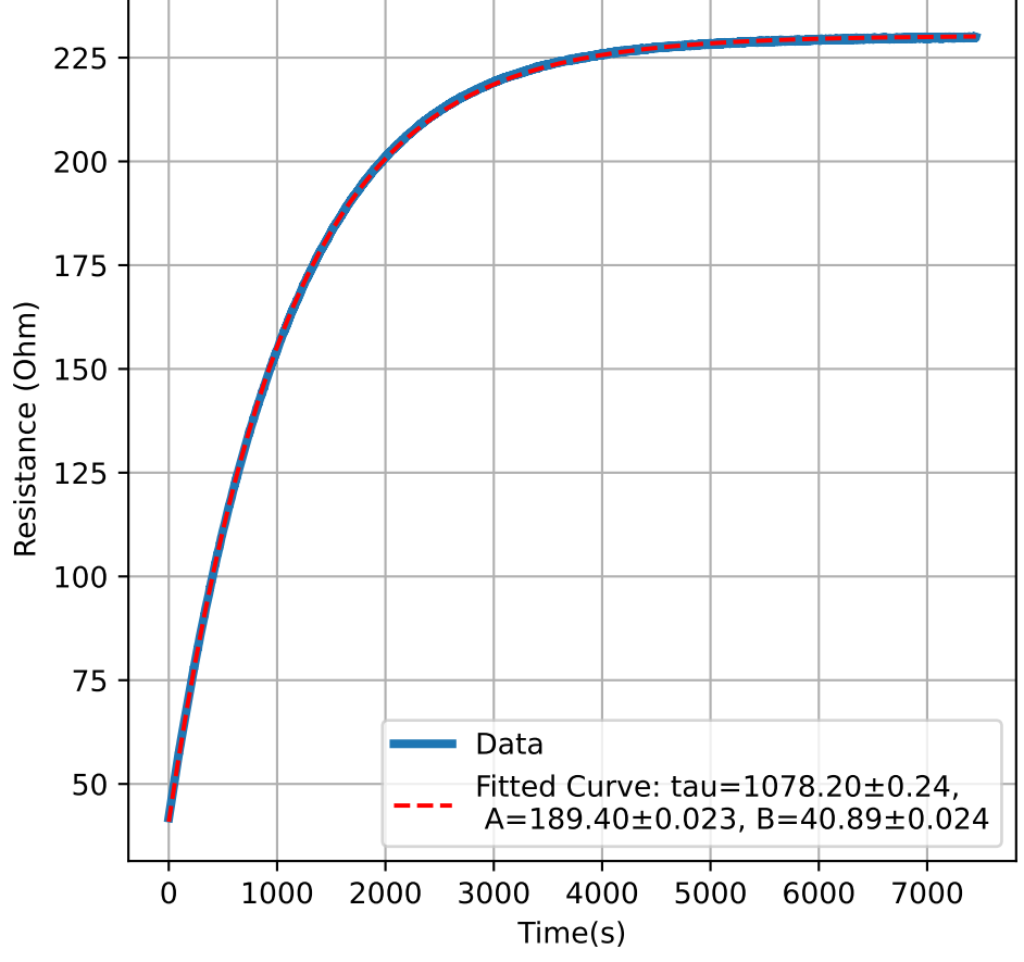
Heater Element 5
