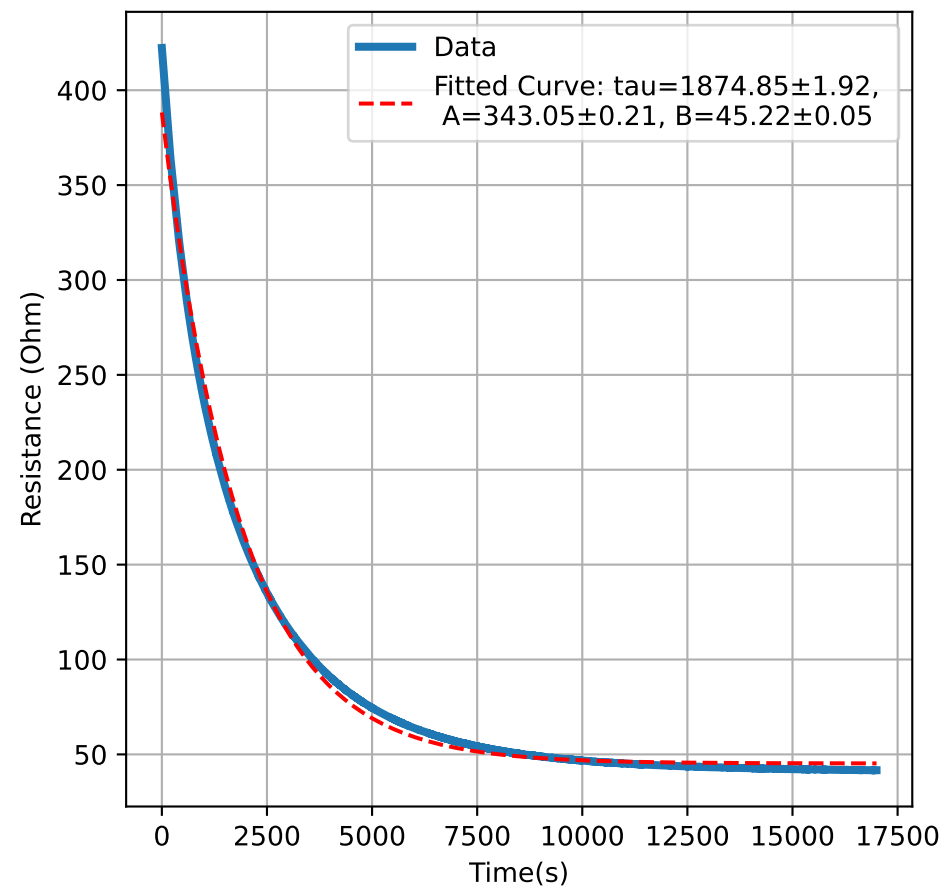
Heater Element 5
