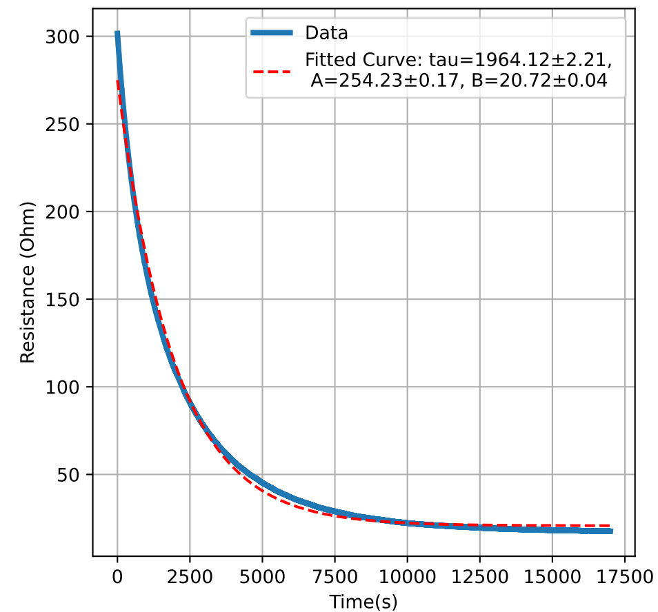
Heater Element 8
