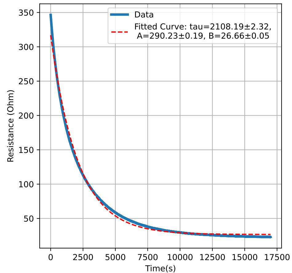
Heater Element 6
