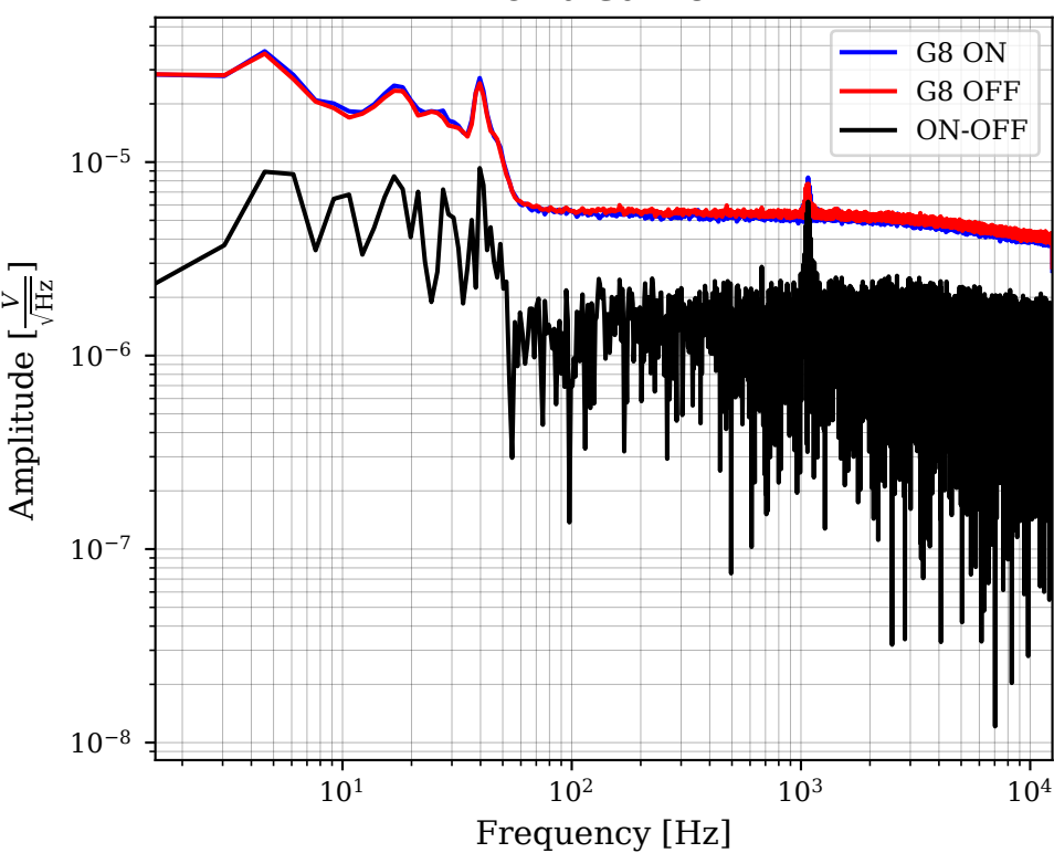
CHO Gain 8
