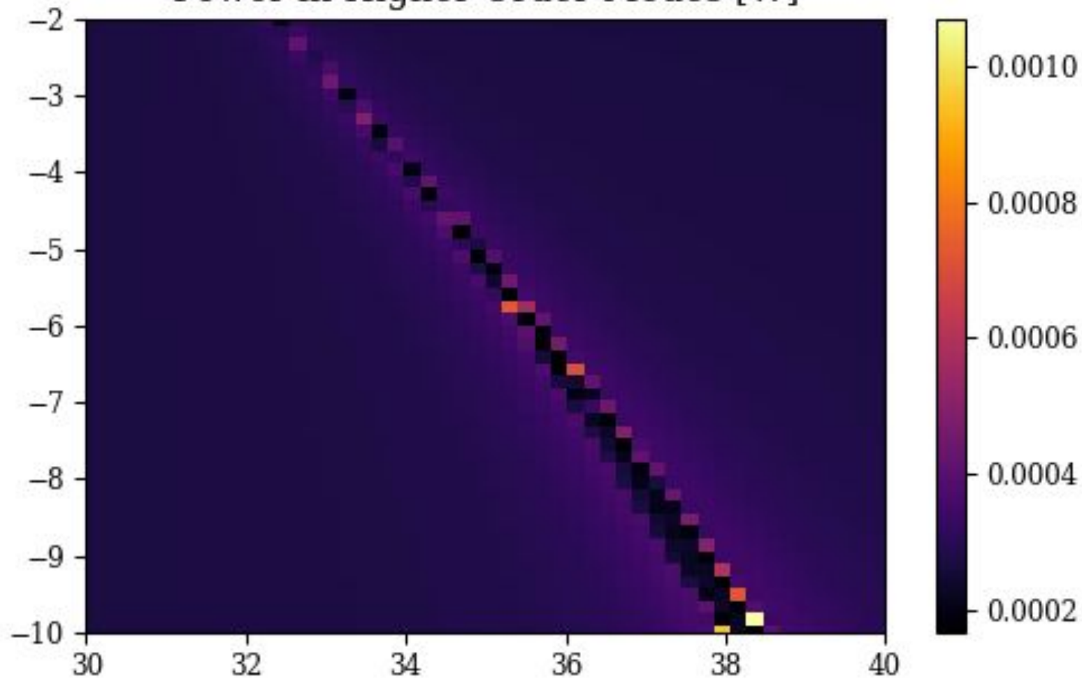
Power in Higher Order Modes [W]
