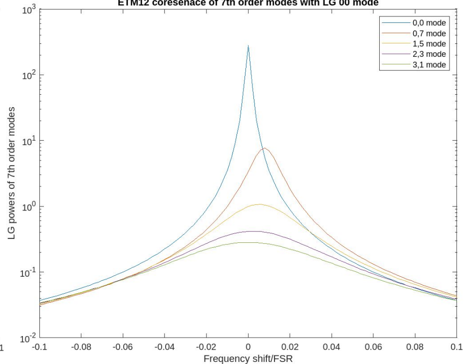
ETM12 coresenace of 7th order modes with LG 00 mode
