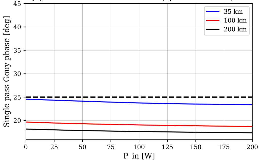
PRC Gouy phase vs initial thermal state (opt. OPD+SURF, ACO2+RH)
