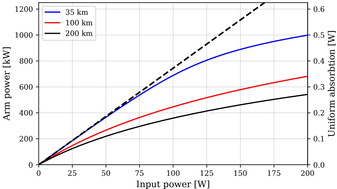
Arm power reached vs initial thermal state ( \alpha = 0.5 ppm, opt. OPD+SURF, ACO2+RH)
