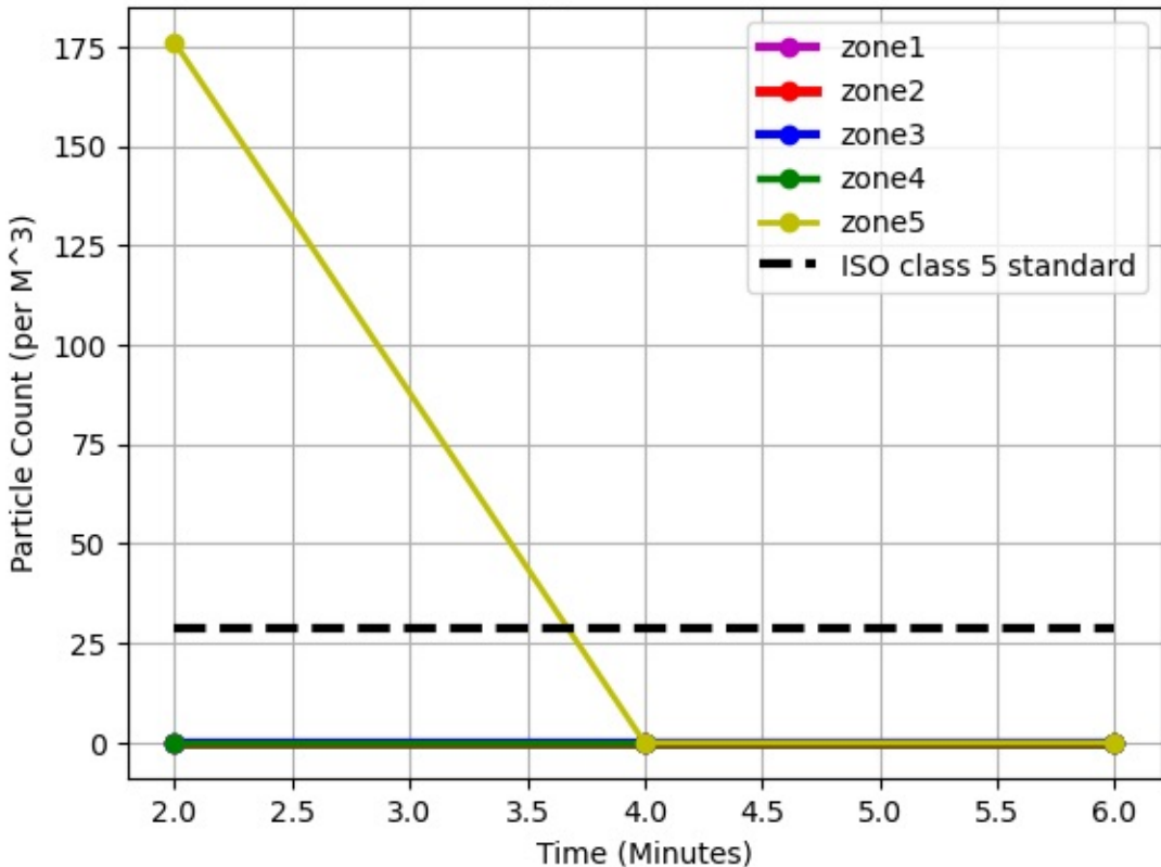
10.0 Microns Range, Unoccupied Clean Room
