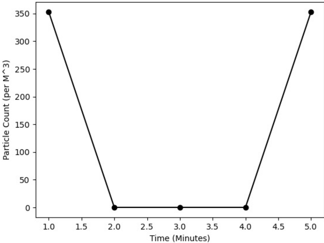
Zone 5, 0.5 Microns
