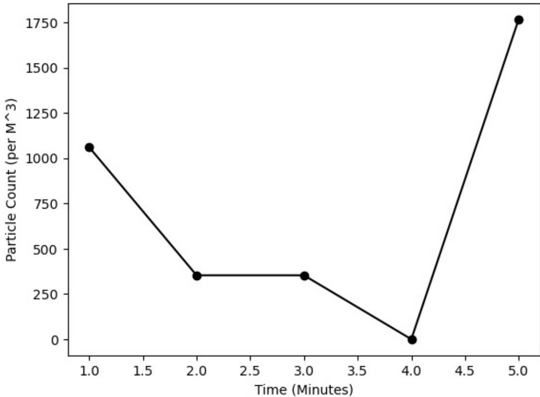
Zone 3, 0.3 Microns
