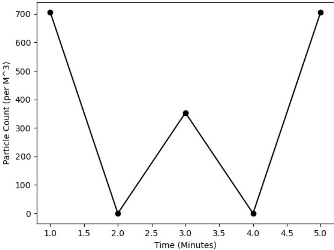
Zone 5, 0.3 Microns
