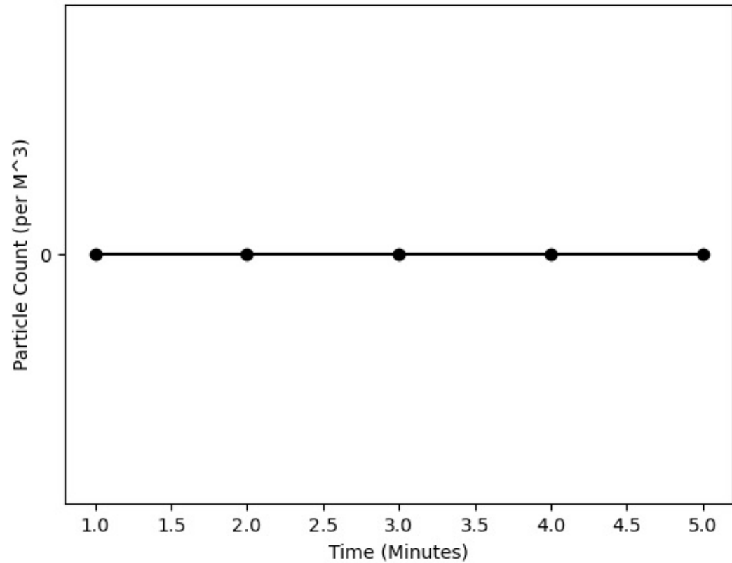
Zone 1, 1.0 Microns
