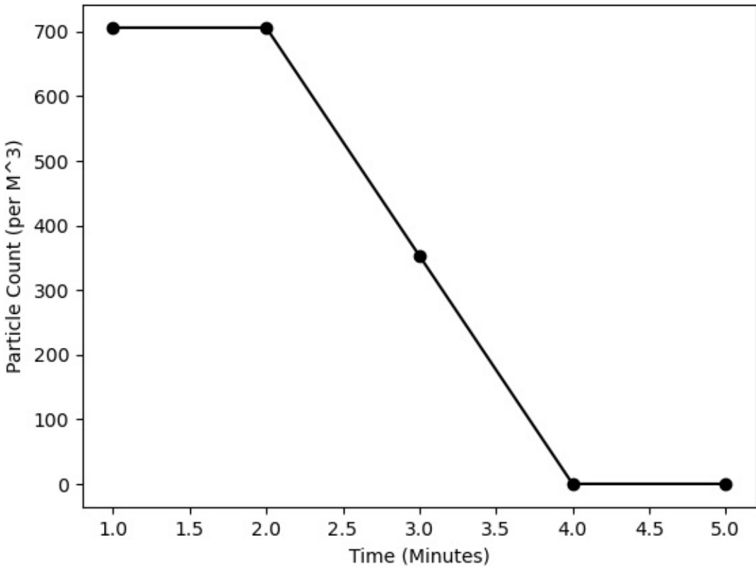
Zone 1, 0.3 Microns
