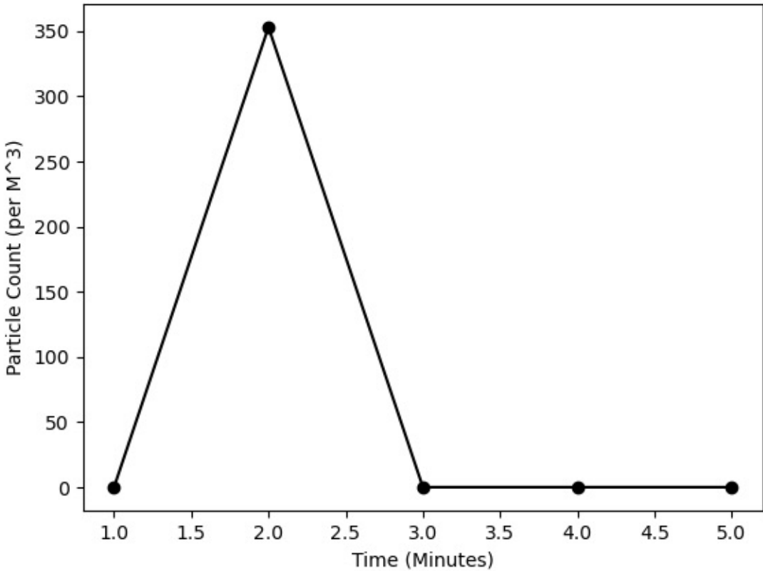
Zone 2, 1.0 Microns
