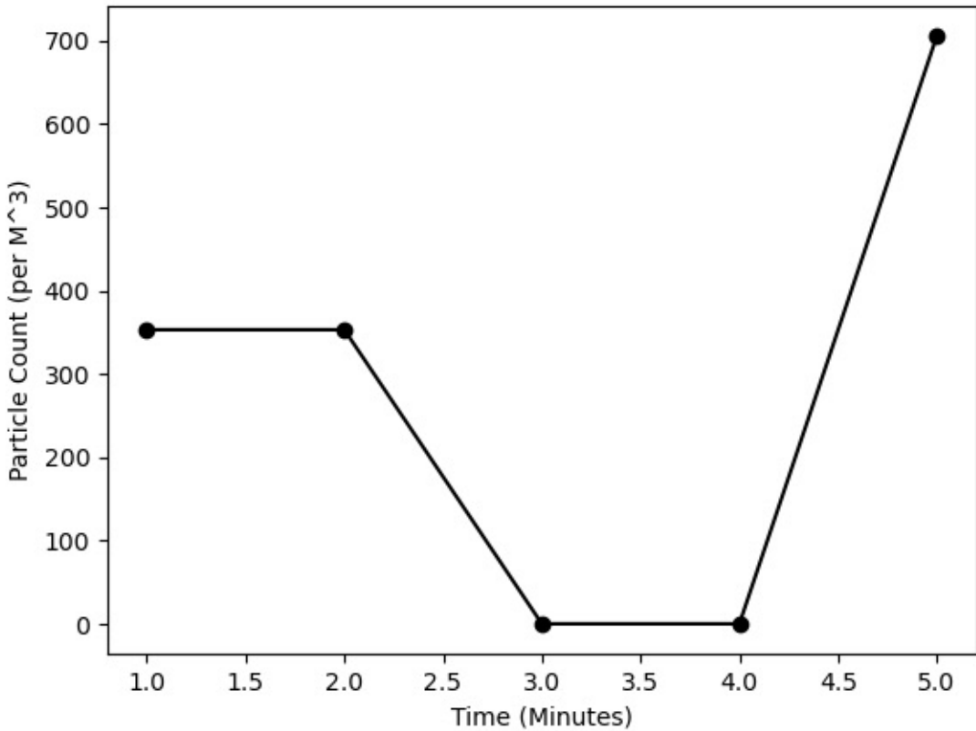
Zone 3, 1.0 Microns
