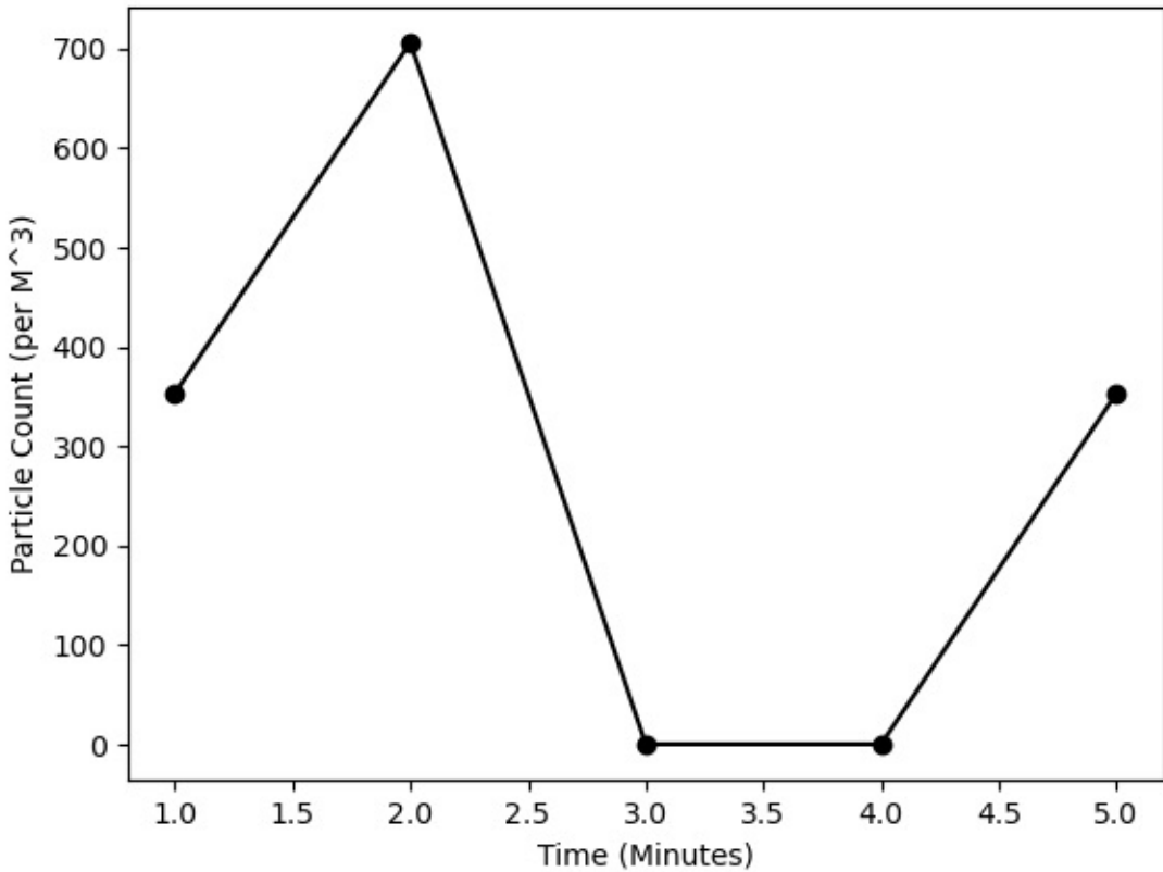
Zone 4, 0.3 Microns
