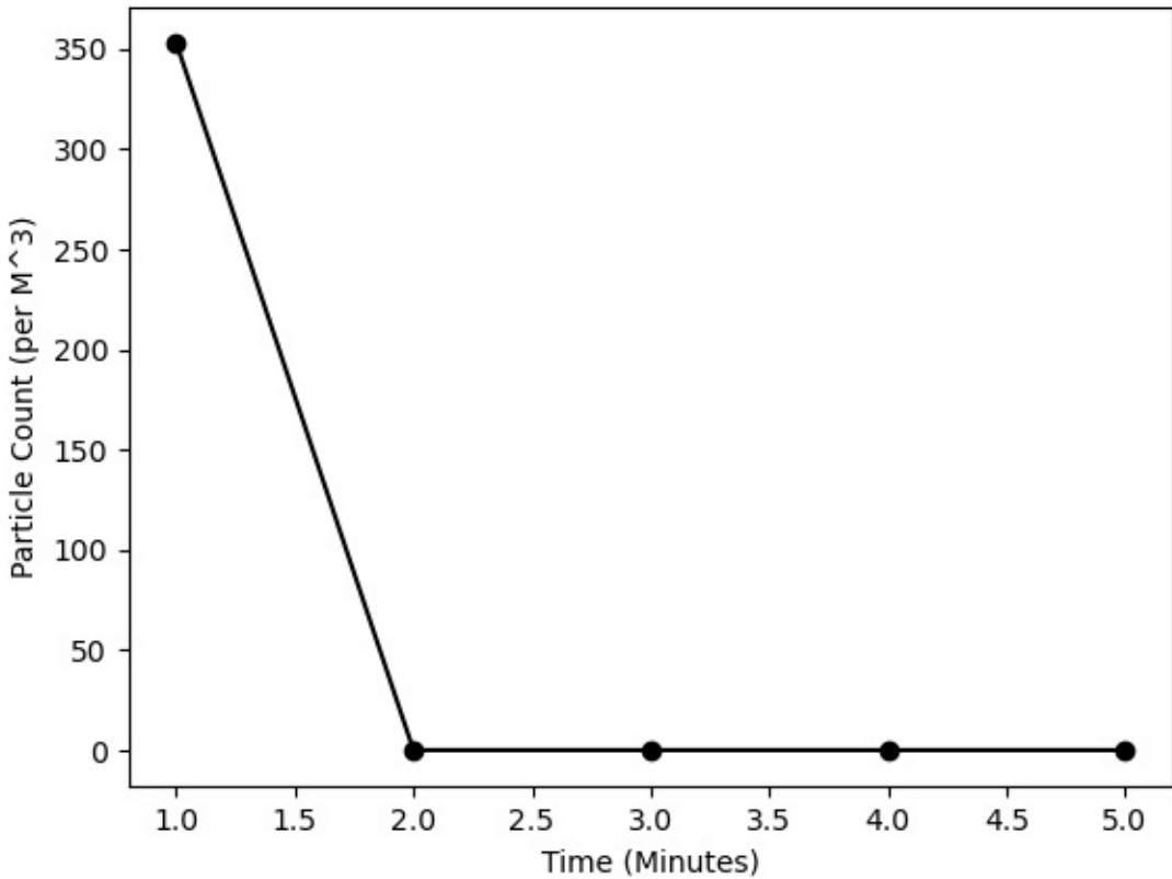
Zone 1, 0.5 Microns
