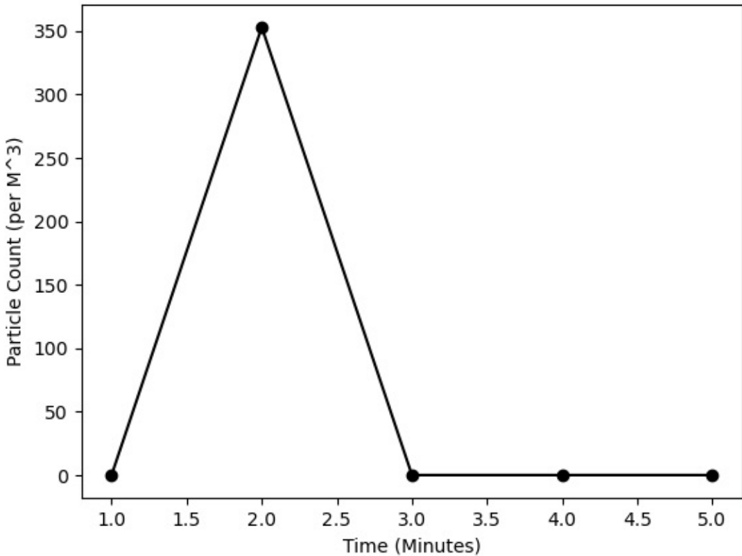
Zone 2, 0.5 Microns
