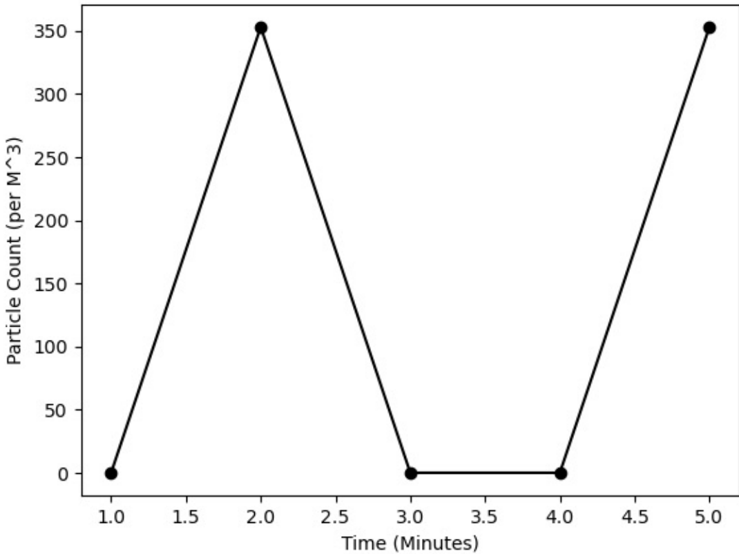
Zone 3, 2.5 Microns
