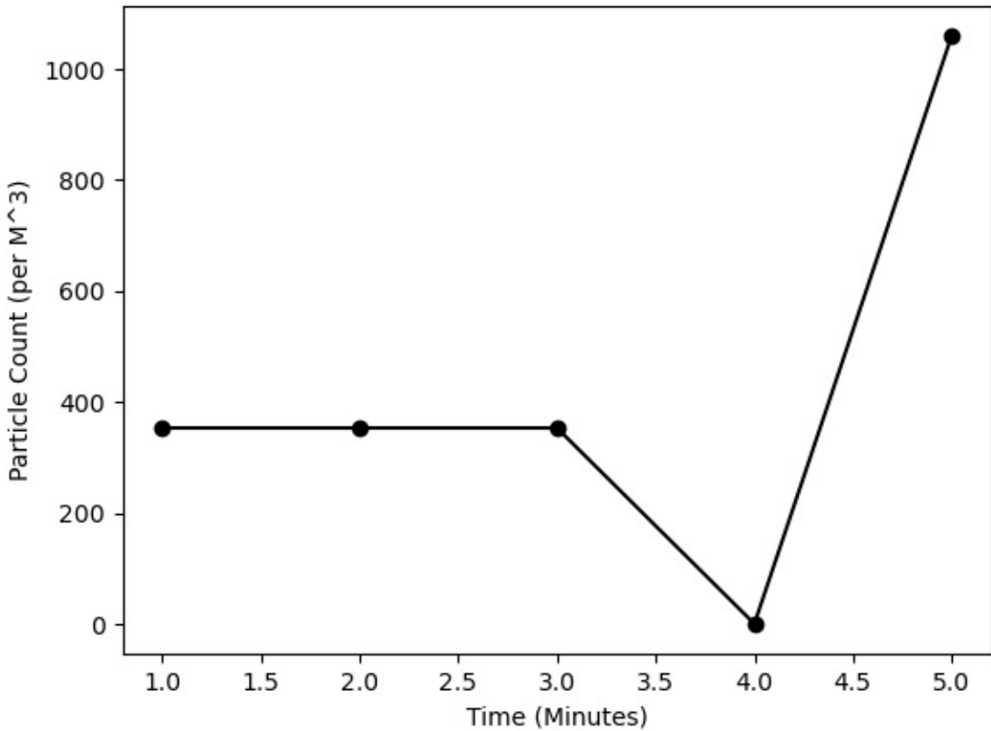
Zone 3, 0.5 Microns
