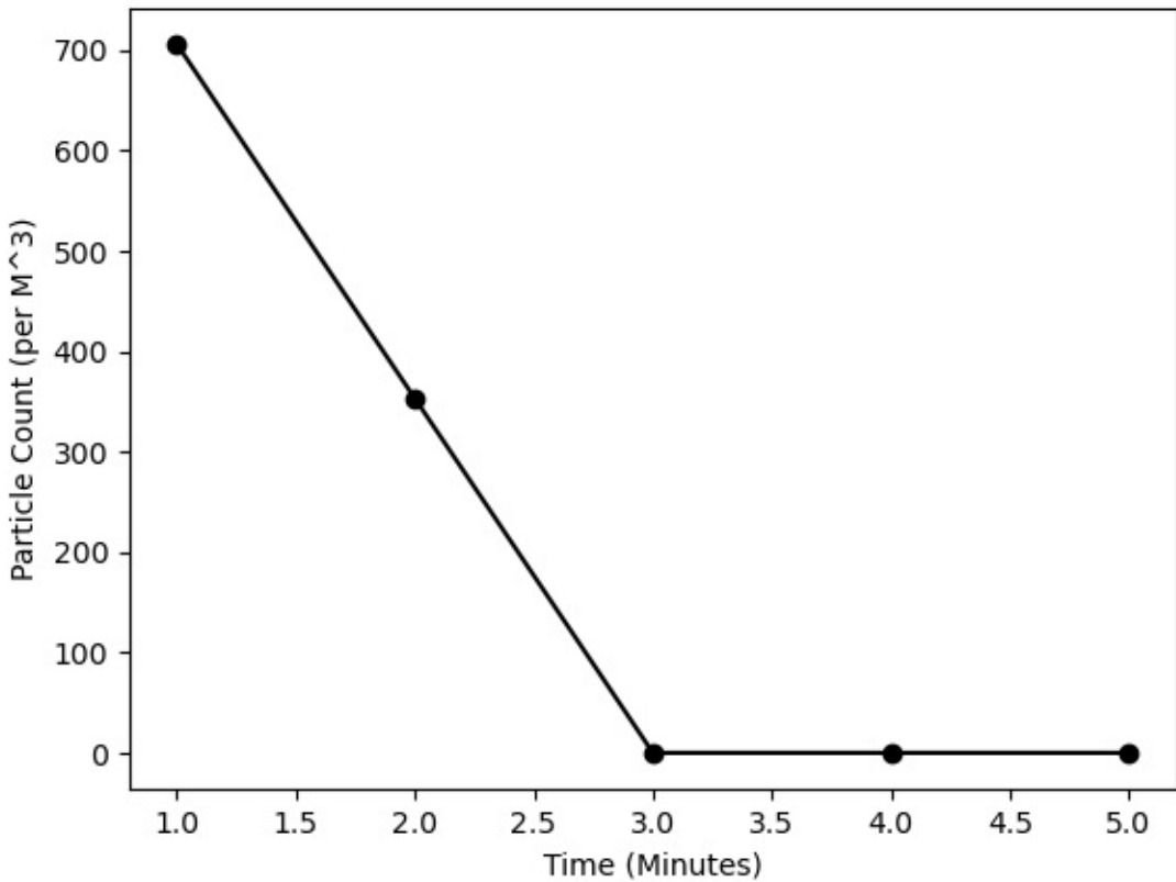
Zone 2, 0.3 Microns
